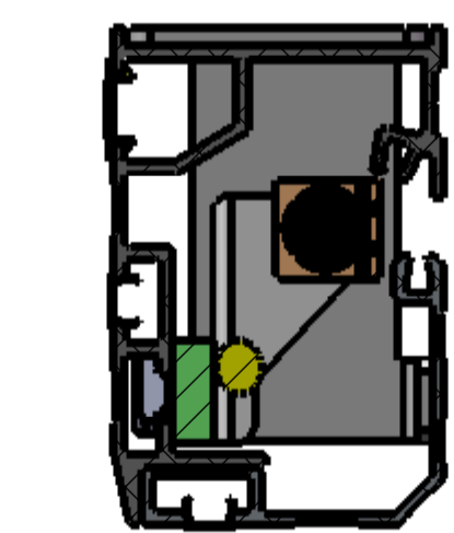
SECTION C-C SCALE 1 : 2
